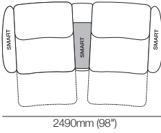
King Cinema Premiere 2.5-Seater 900R MEDIA SMART Top View
