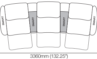
King Cinema Premiere 3-Seater 800R MEDIA SMART Top View
